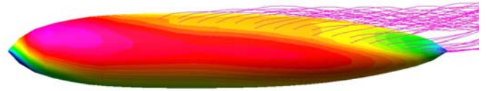
U.S. Airship Akron showing Body Vortex at Angle of Attack and Boundary Layer Velocity Profiles
